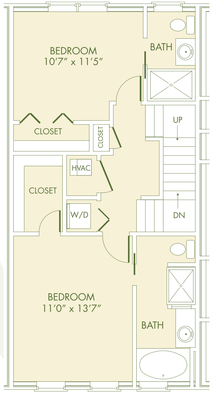
SECOND FLOOR
